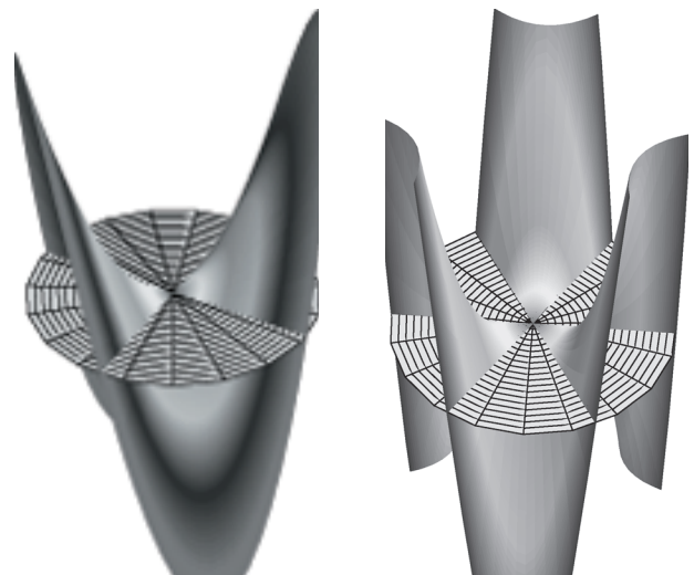
FIGURE 4 Gaussian Surfaces
