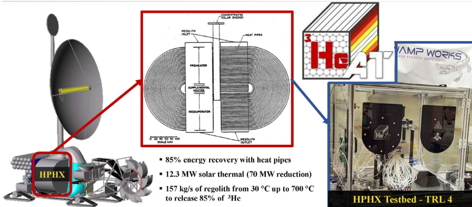
FIGURE 10 Helium Extraction & Acquisition Testbed (HEAT) Concept
