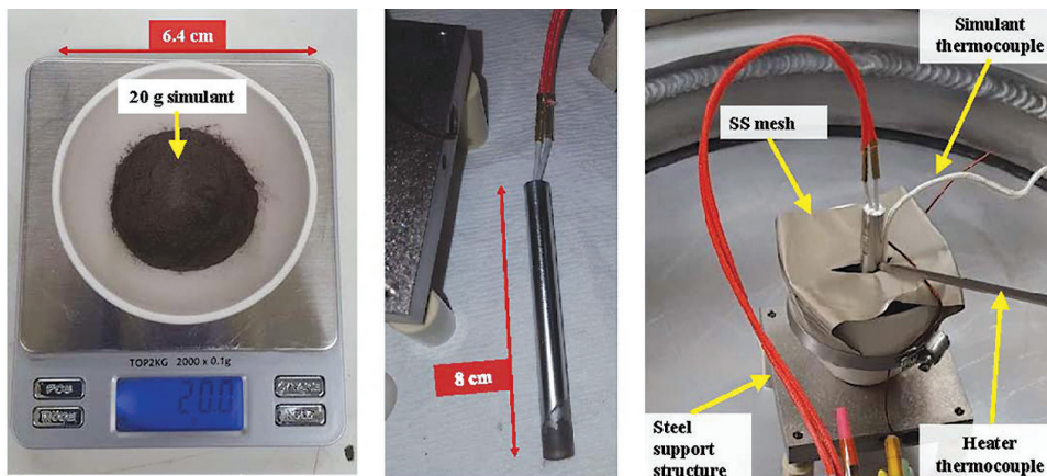
FIGURE 11 Sample Concentration Analyzer (SCAN) Components
