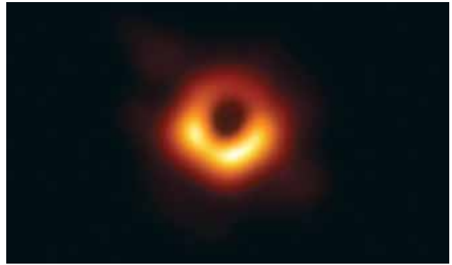
EHT First-ever picture of a supermassive black hole candidate's environment. The center of galaxy Messier 87, as imaged by the Event Horizon Telescope in April 2017.
