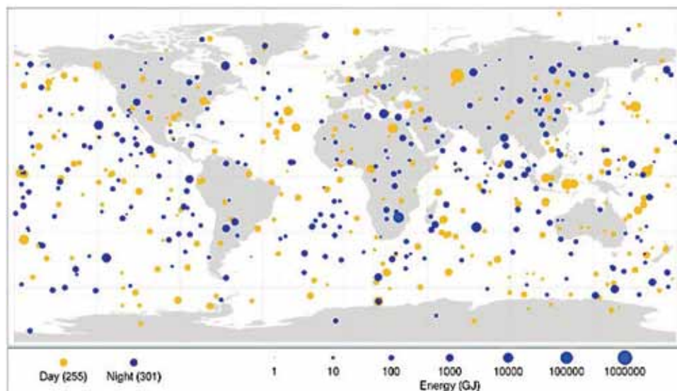
FIGURE 2 Bolide events 1994-2013
