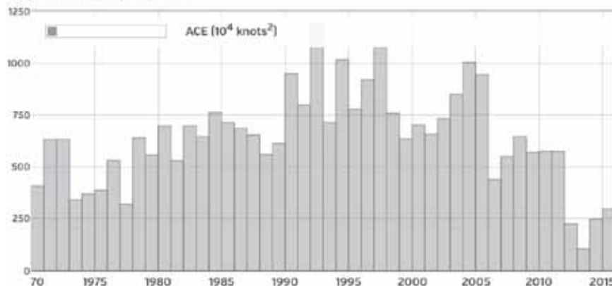
Accumulated Cyclonic Energy (ACE), a measure of the energy components of storms, has tended to decrease for the last 15 years, while CO 2 emissions have risen.
