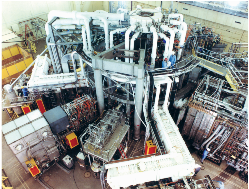
The Tokamak Fusion Test Reactor at Princeton. The TFTR operated from 1982 to 1997, setting many significant records both in plasma temperature and in peak fusion power produced, before it was prematurely shut down.
