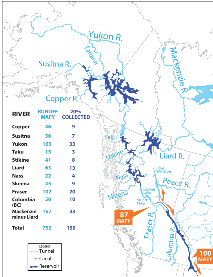
FIGURE 4 Northern Collection System
