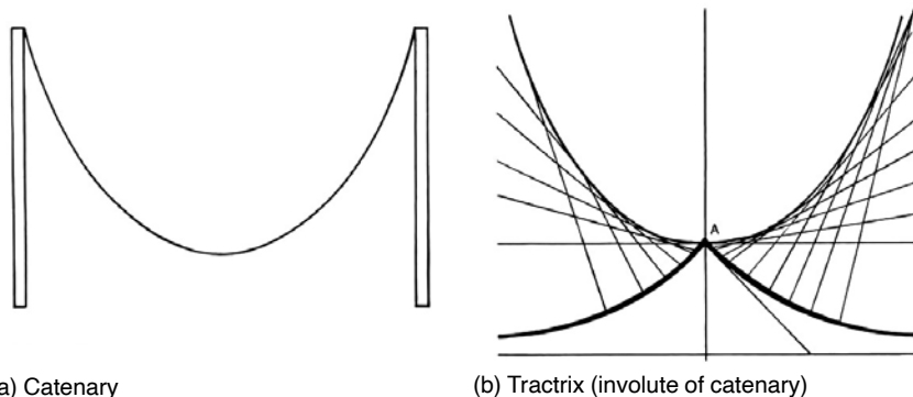
(a) Catenary
